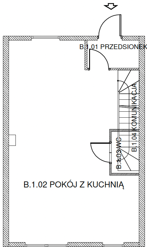
PARTER - 49.47 [m2]
