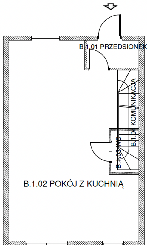
PARTER - 49.51 [m2]
